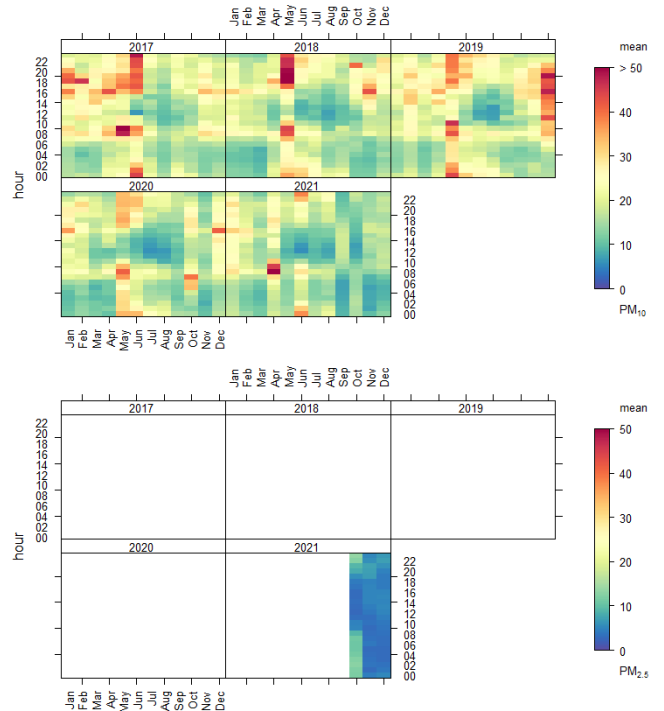
Figure 3 Average PM 10 (upper) and PM 2.5 (lower) concentrations at Collie for each hour over the last five years
