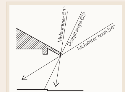
Figure 70: Calculated eaves overhang on north side, Perth.
