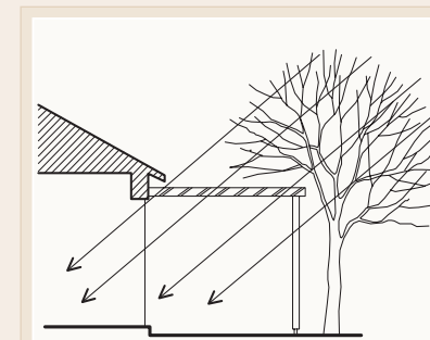
Figure 69: Solar pergola and deciduous trees.
