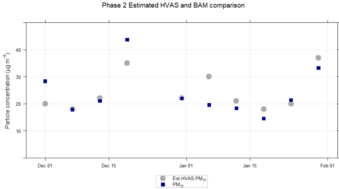
Figure A1-5 Phase 2 HVAS and BAM daily PM 10 comparison
