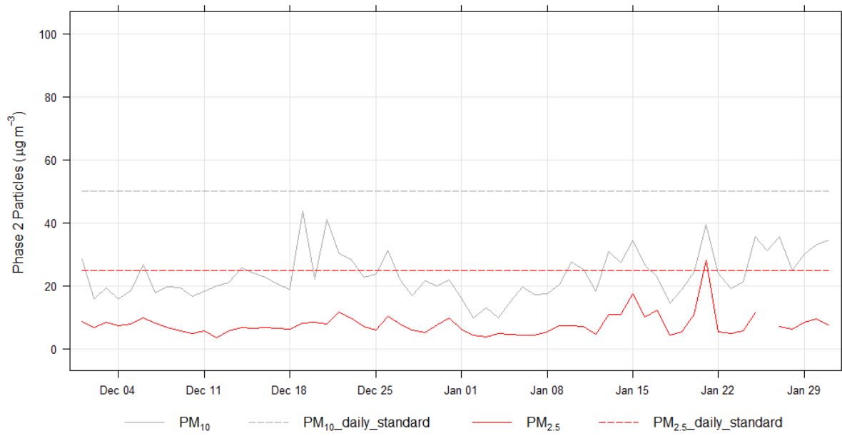
Figure A1-4 Phase 2 BAM daily PM_{10} and PM_{2.5} concentrations and NEPM guidelines
