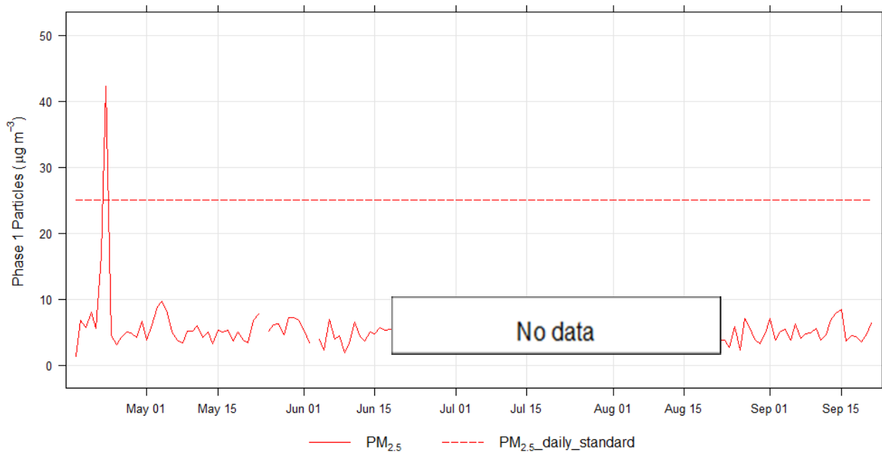
Figure A1-2 Phase 1 BAM daily PM_{2.5} concentrations and NEPM guideline ( 25 \mu\text{g}/\text{m}^3 )
