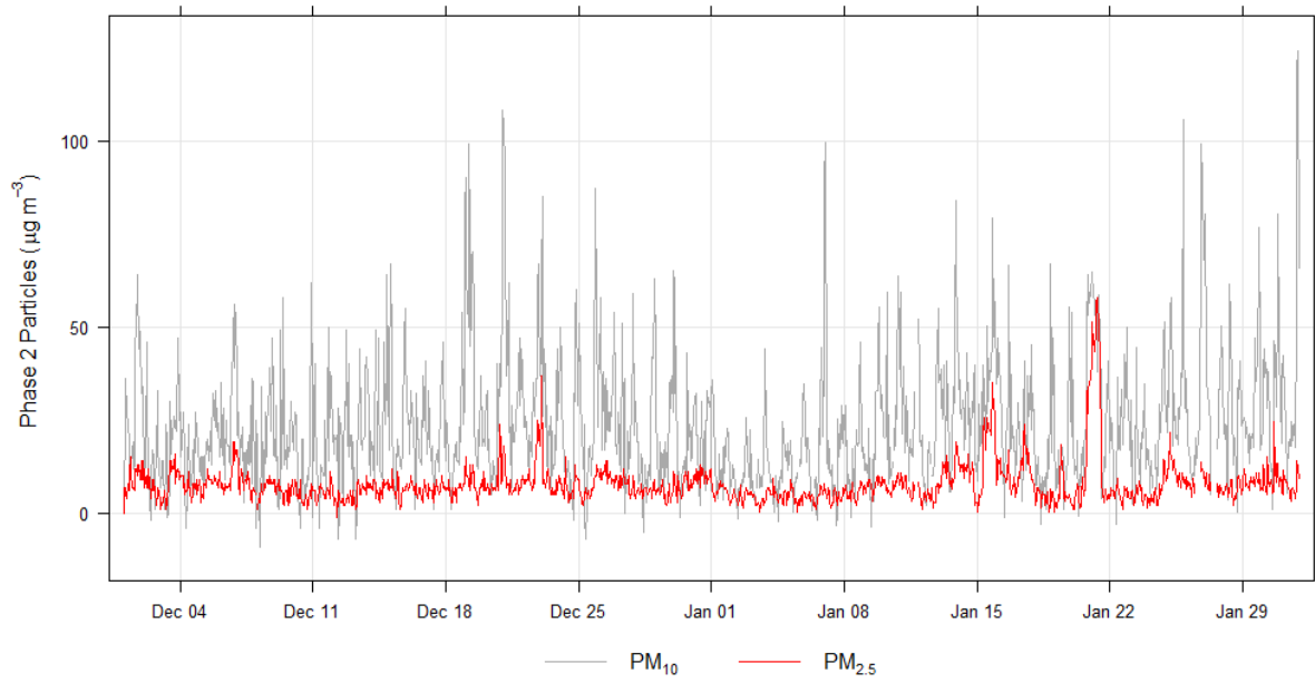
Figure A1-3 Phase 2 BAM hourly PM_{10} and PM_{2.5} concentrations
